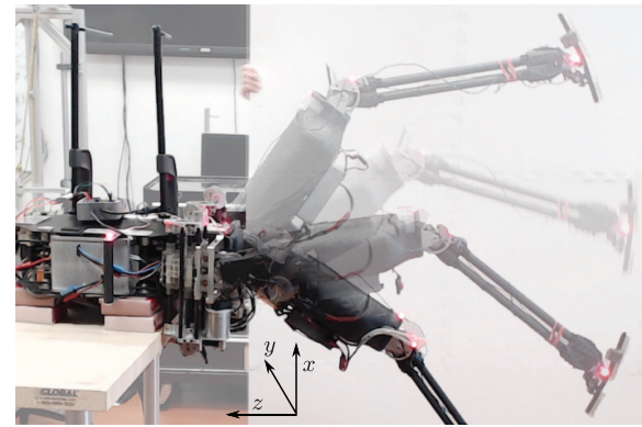
(a) Kinematics calibration test
