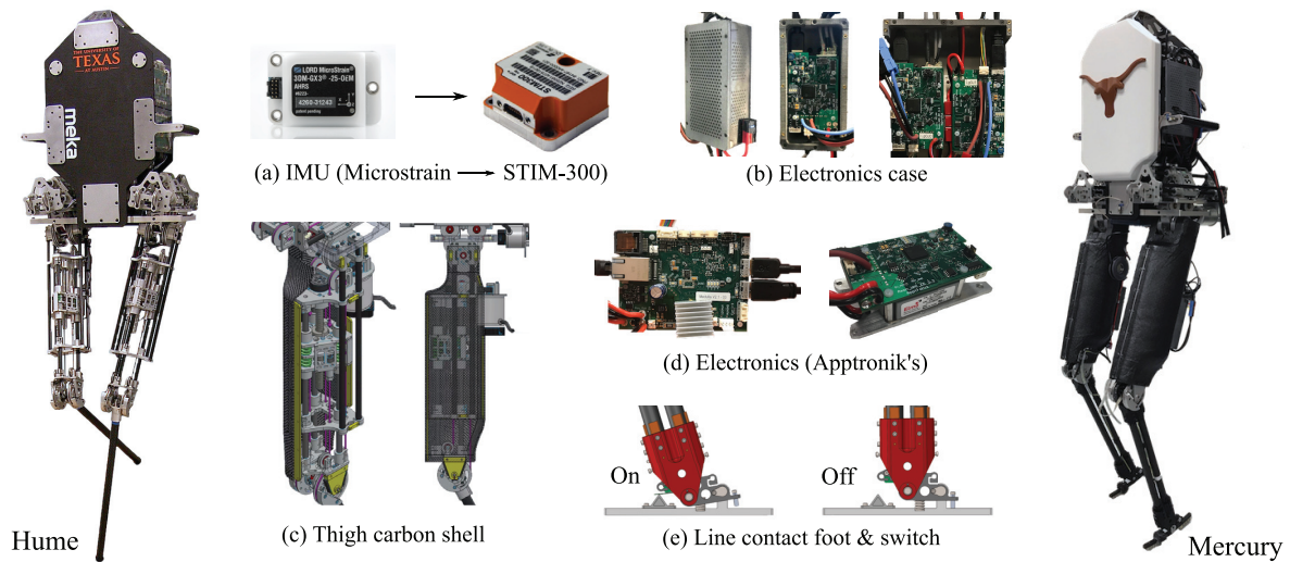
Fig. 2. Hardware upgrades of Mercury. (a) The IMU was upgraded to the Sensoror's STIM-300, which has low angular velocity drift and bias, enabling accurate orientation estimates even with simple forward integration. (b) The on-board electronics have been installed with cases to secure the electric cables in place. Keeping the cables in place significantly reduces losses of connections and cable damage during robot operations. (c) Carbon fiber cases were installed on Mercury's thighs to increase structural stiffness. (d) All of the embedded electronics were replaced with Appttronik's Medulla and Axon boards that come with a variety of low-level controllers for SEAs. (e) Spring-loaded passive ankles with limit switches were also added to limit the uncontrollable yaw body rotation and detect ground contacts.
